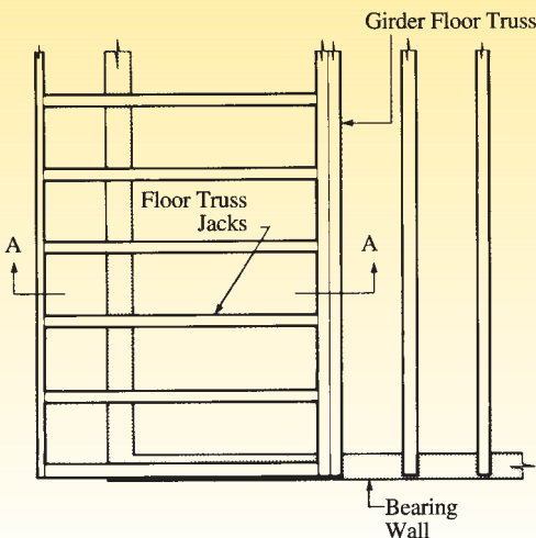
Floor Cantilevered Perpendicular to Floor Truss Span
