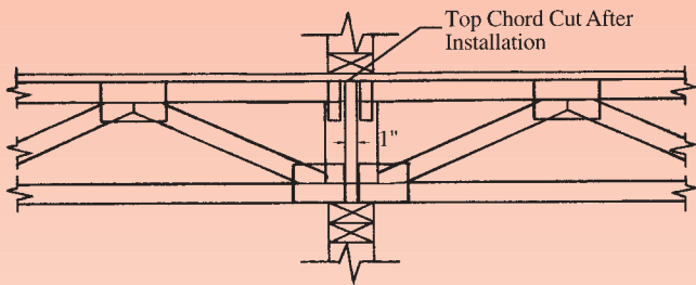
Intermediate Bearing - Simple Span Trusses
