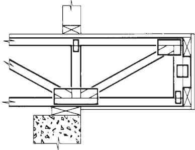
Balcony Cantilever
