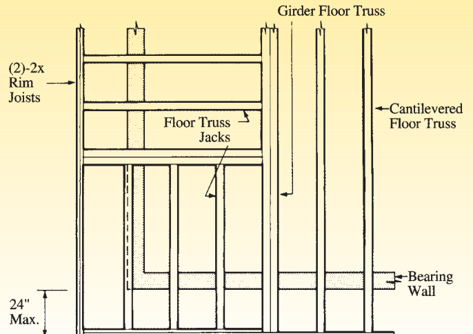
Floor Cantilevered Perpendicular and Parallel to Floor Truss Span
